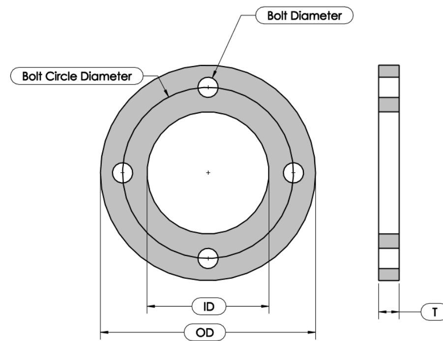
ASME B16.21 GASKET DIMENSIONS FOR ASME B16.5 150# FLANGE (INCHES)
