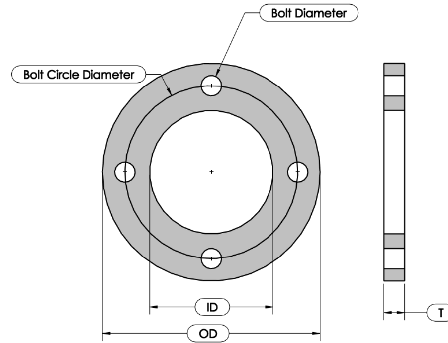
ASME B16.21 GASKET DIMENSIONS FOR ASME B16.5 150# FLANGE (MM)
