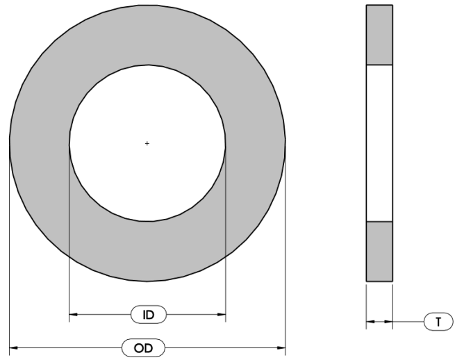
ASME B16.21 GASKET DIMENSIONS FOR ASME B16.5 FLANGE (INCHES)
