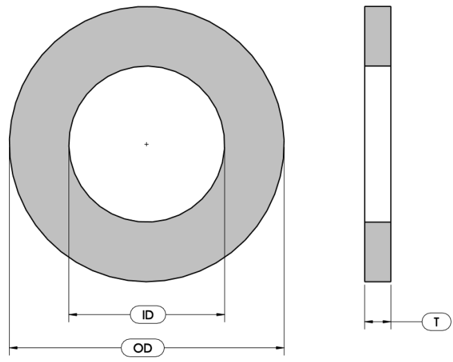
ASME B16.21 GASKET DIMENSIONS FOR ASME B16.5 FLANGE (MM)
